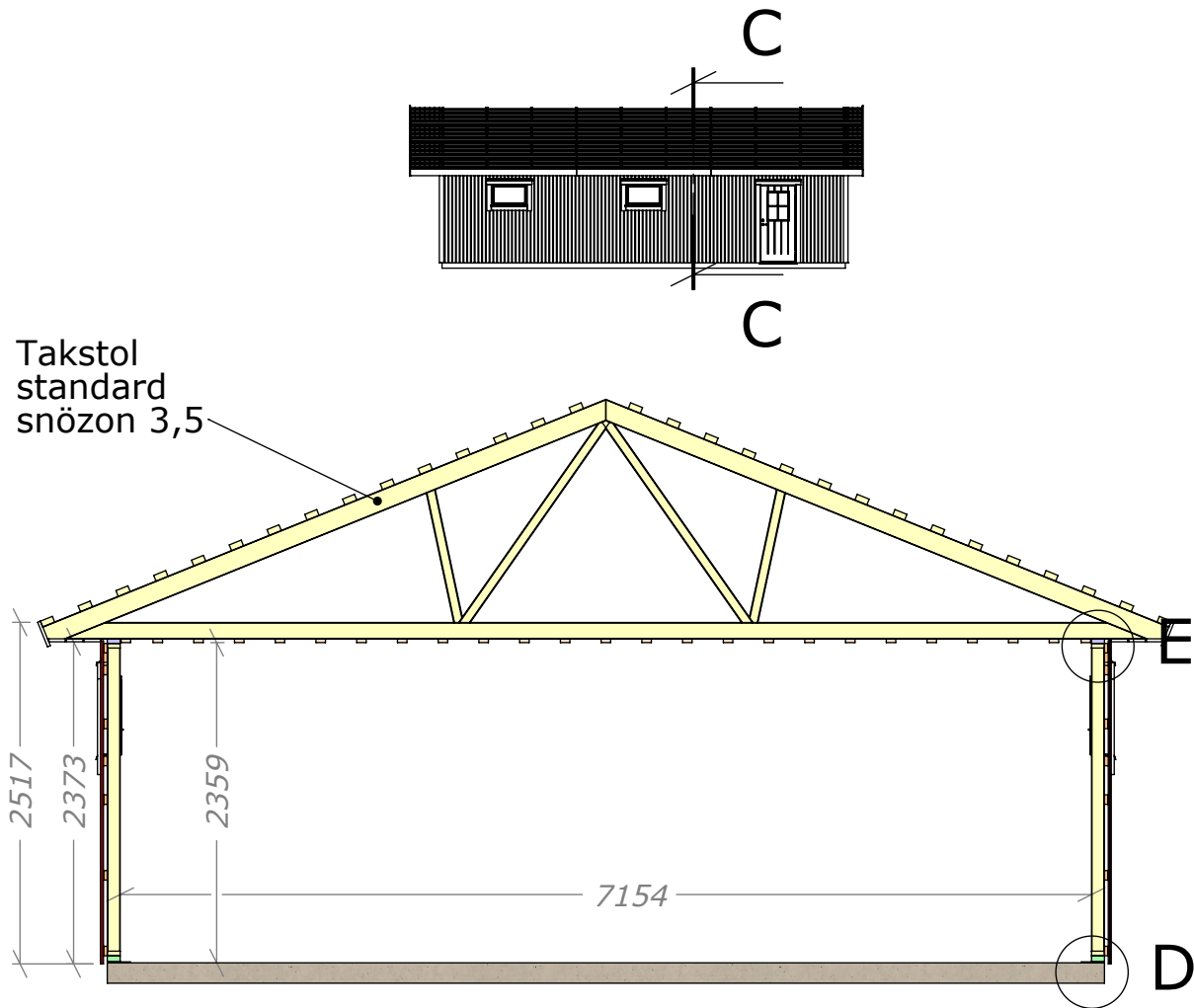
SECTION C-C SCALE 1 : 55
