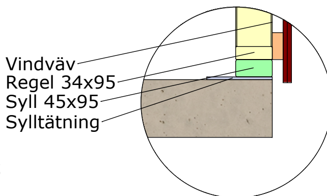
DETAIL D SCALE 1 : 10
